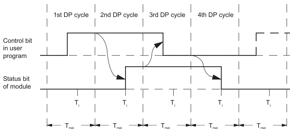
Figure 2-42 Acknowledgment Principle in Isochrone Mode
