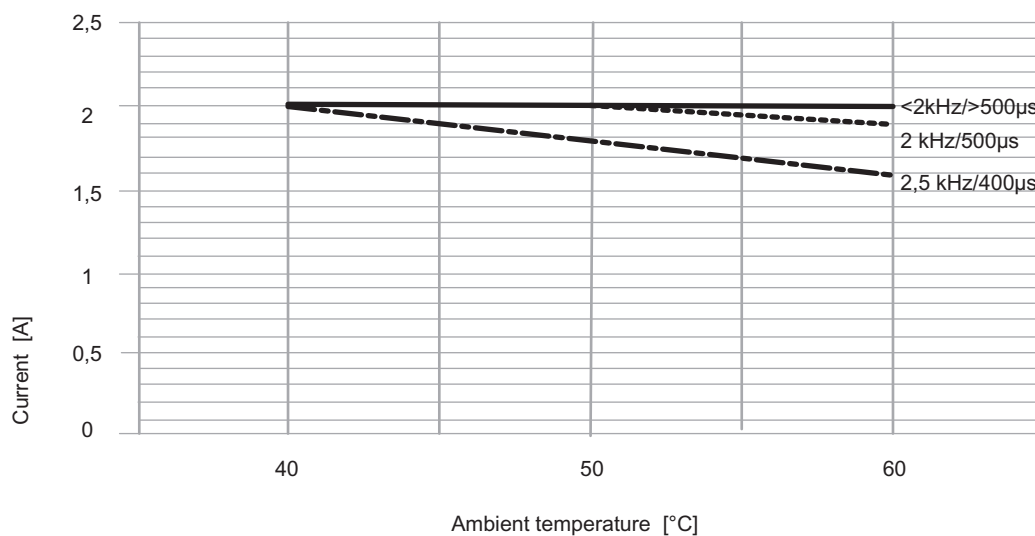
Figure 5-30 Resistive Load - Only Channel 1 PWM 50/50
