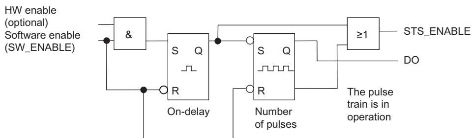
Figure 5-8 Basic Circuit Diagram for Pulse Train Mode
