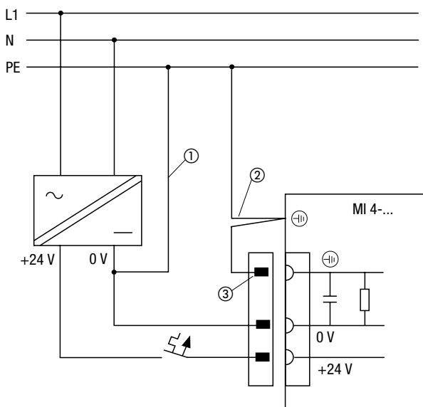
Figure 1: Connection diagram
