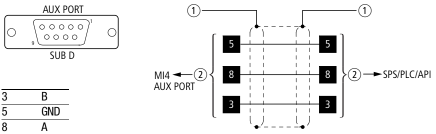
Figure 6: Siemens MPI communication cable
